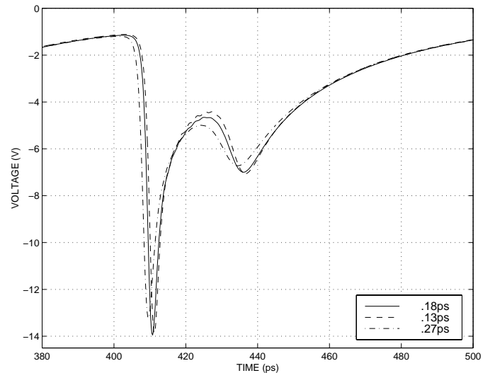
Fig. 10. Comparison between simulations using different time steps
