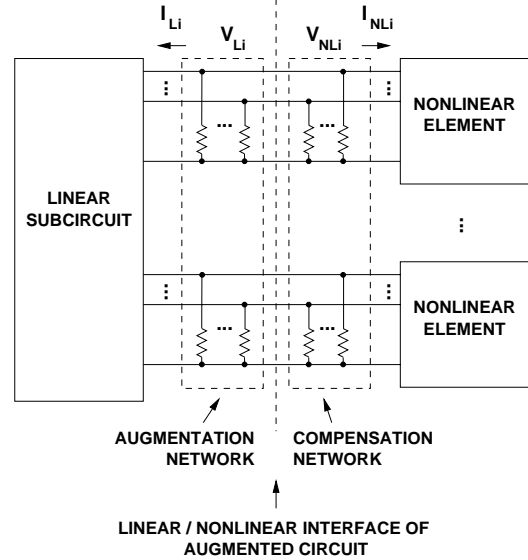
Fig. 2. Augmentation and compensation network
