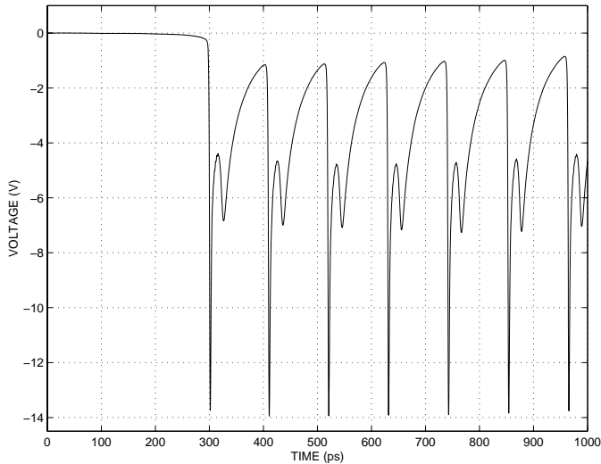
Fig. 7. Complete transient response for the soliton line
