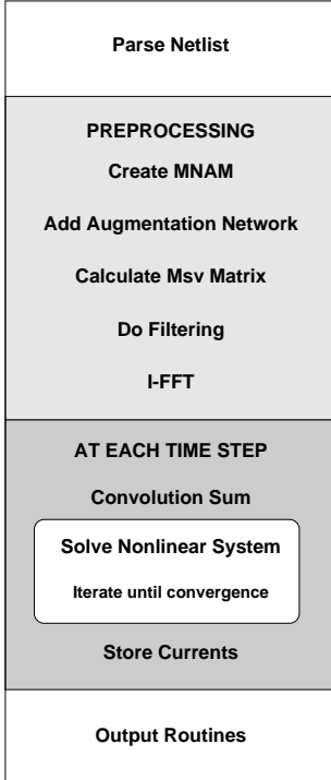
Fig. 1. Flow diagram of the analysis code
